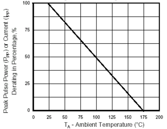
Fig.2-Power Derating Curve
